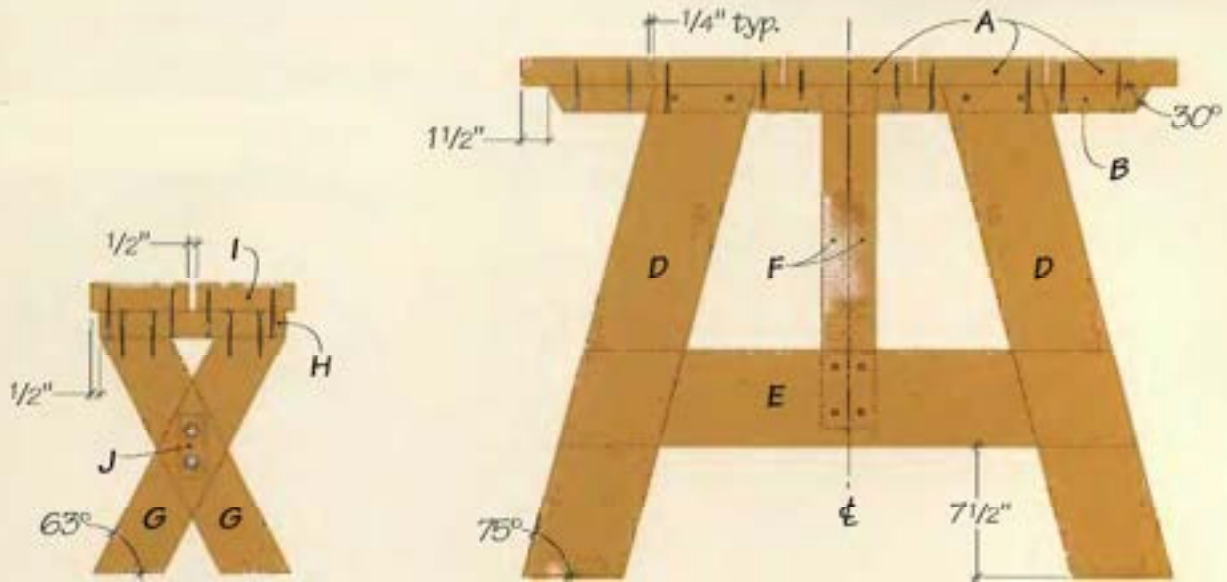
BENCH END VIEW
