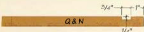
DRAWER SIDES (Q & N)
