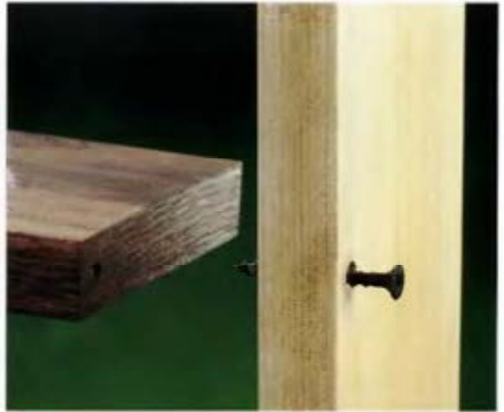
A BUTT JOINT can be used in just about any woodworking situation. If it will undergo stress or pressure, it's a good idea to reinforce the glued butt joint with a fastener, such as a screw.
