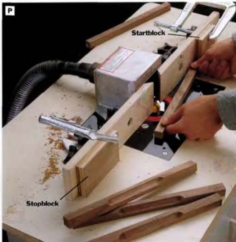
PHOTO P: Rout cove-shaped finger pulls into the undersides of the handles using a router table fitted with a \frac{3}{8} -in. core box bit. Clamp a start block and a stopblock to the table fence to guide your cuts.
