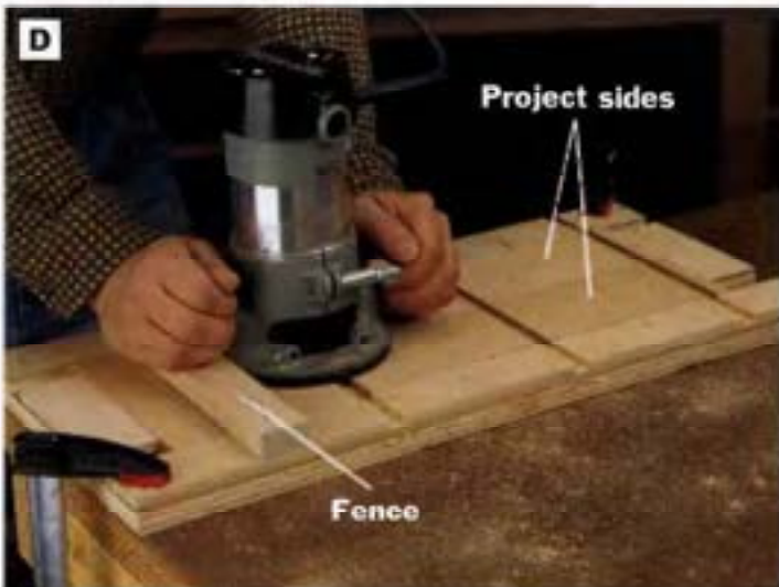
PHOTO D: Create a simple shop-made jig out of plywood to gang-rout shelf dados across the sides. Guide the router base along a removable fence, and rout each dado clear across both the jig and sides.
