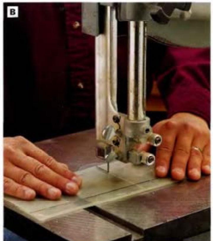
PHOTO B: Measure and cut the Plexiglas end panels on the band saw with a fine-toothed blade. Leave the protective film on the plastic as you machine it, to minimize scratching.
