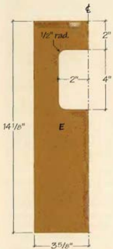
BACK (E)
