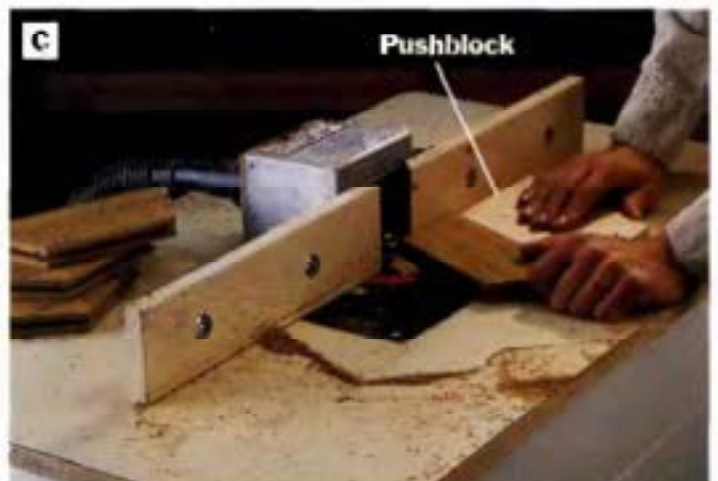
PHOTO C: Rout spline grooves in the angled ends of the tabletop rails. Use a pushblock to aid in running the narrow pieces across the cutter and to back up the cut, preventing chipout.
