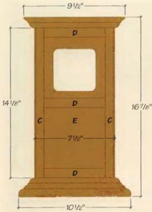
FRONT VIEW
