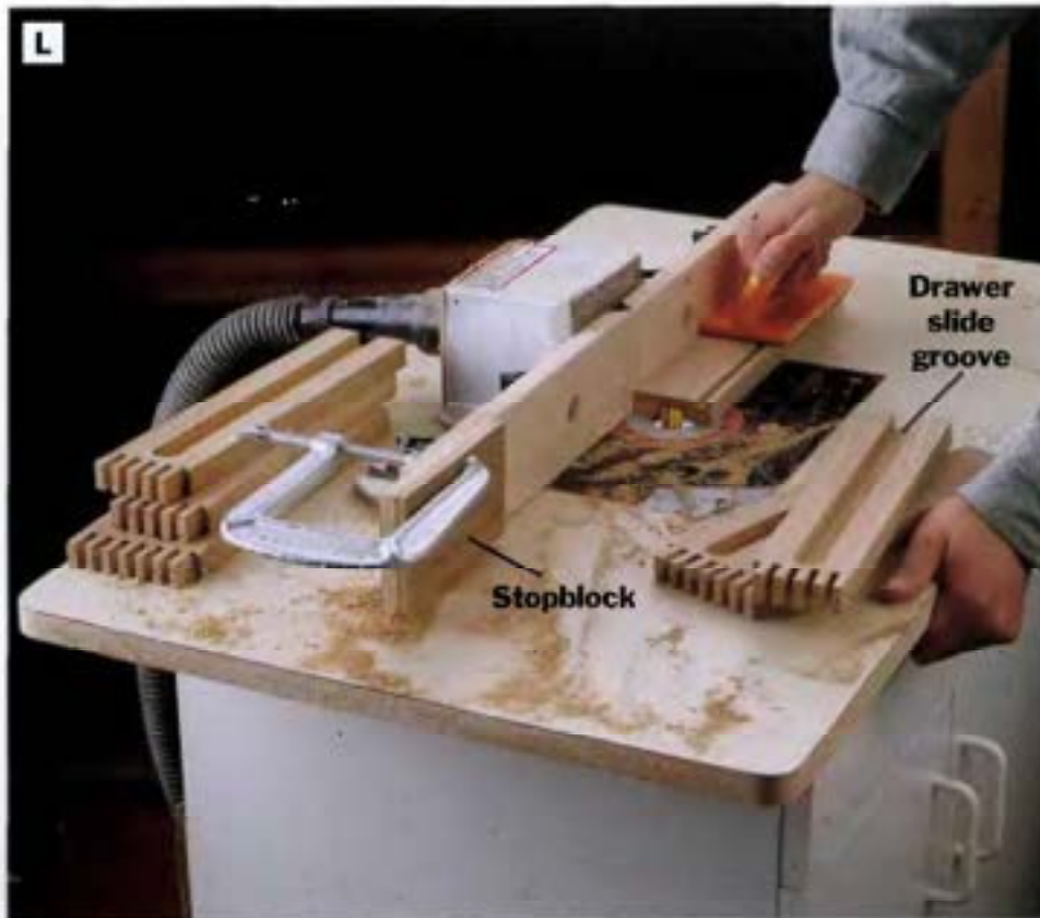
PHOTO L: After the drawer bottom grooves have been cut on the router table, rout grooves for the drawer slides. Both are stopped dados, cut in multiple passes.
