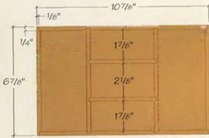
TRAY TOP VIEW
