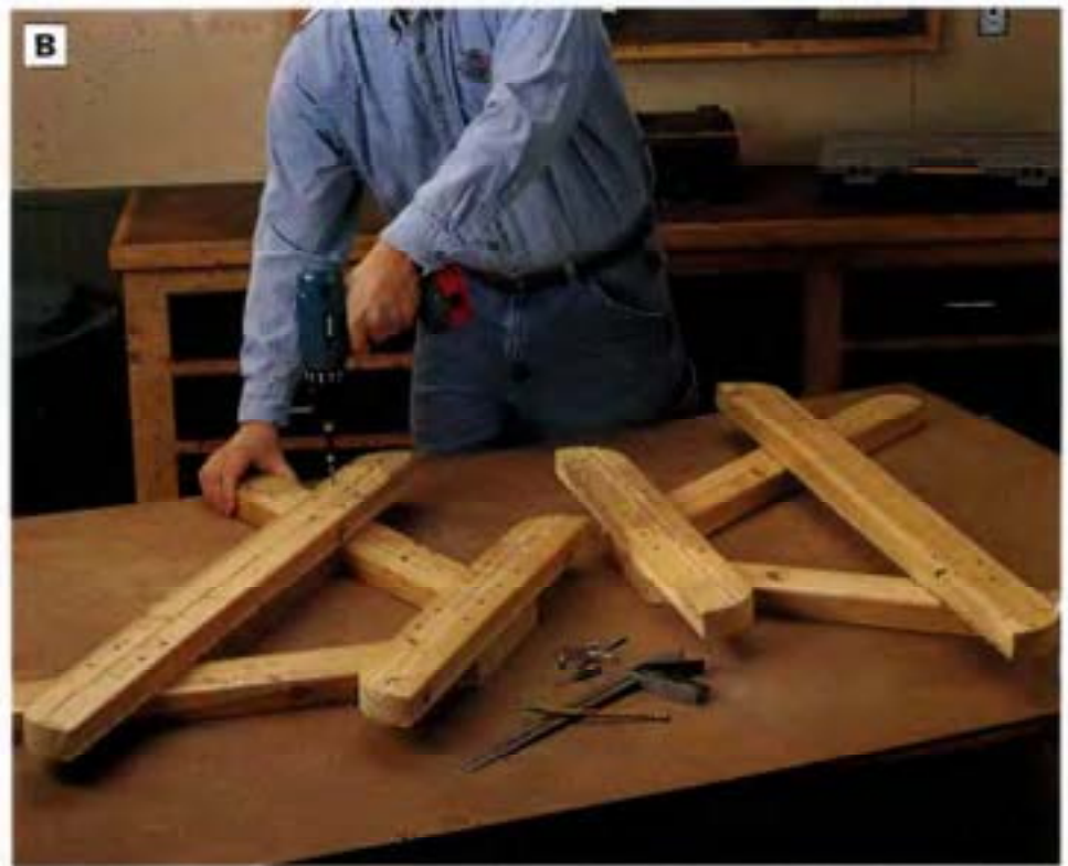
PHOTO B: Set pairs of legs on your worksurface so they splay outward with their angled ends aligned. Attach the top stringers flush to the tops of the legs, and install the seat stringers so they overhang the legs by 8 in. on each end. Fasten the parts with countersunk 2\frac{1}{2} -in. deck screws to form two leg assemblies.
