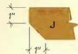
TOP CLEAT END LAYOUT
