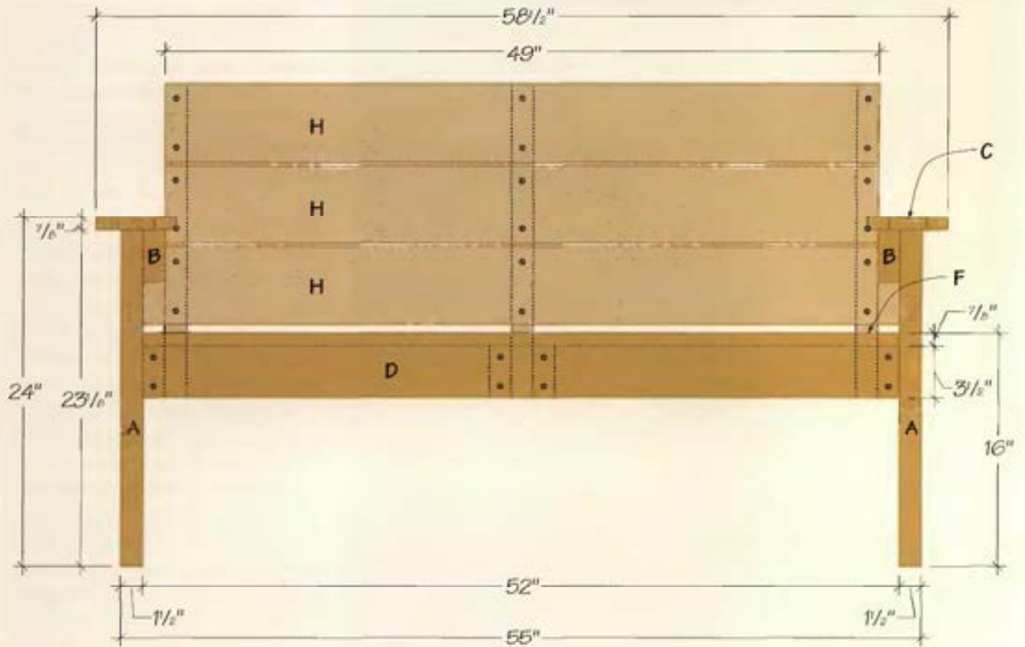
FRONT ELEVATION
