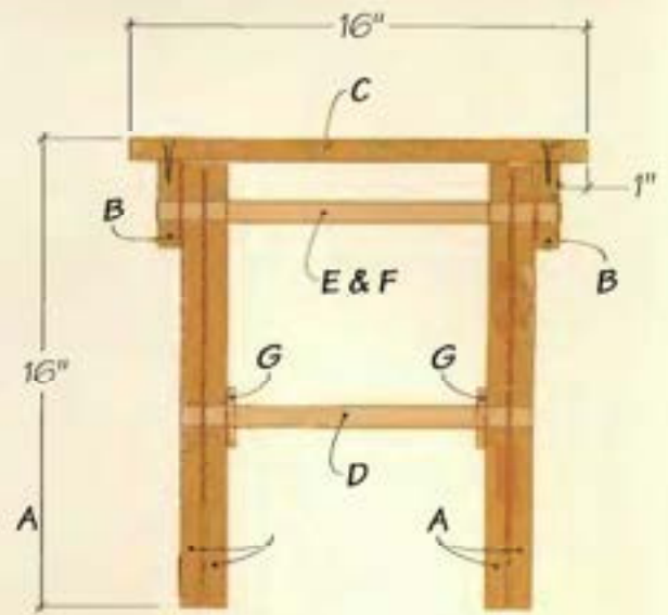
END VIEW
