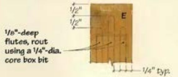
FACE FRAME STILE FLUTING
