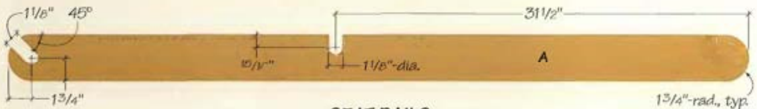
SEAT RAILS
