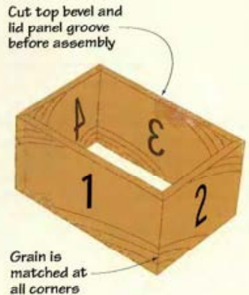
ASSEMBLED BOX
