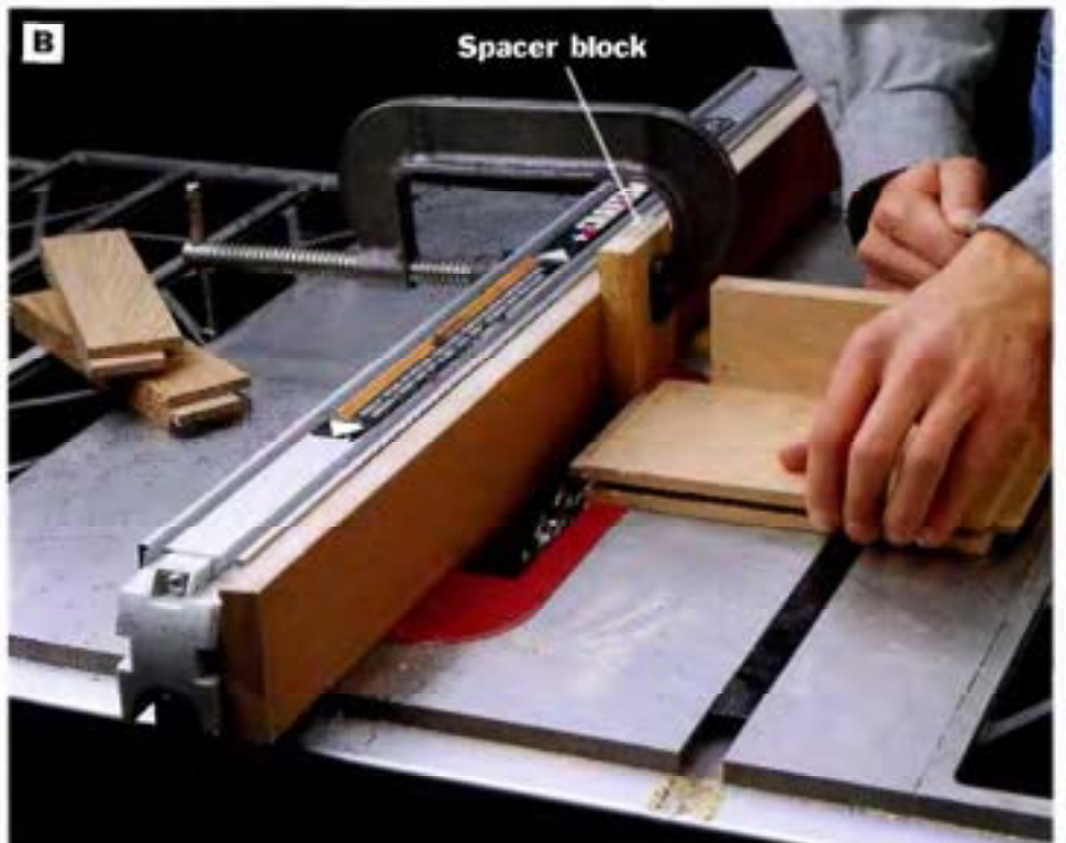
PHOTO B: Cut tenons in the ends of the side and back rails. Use the miter gauge to push the stock and clamp a spacer block to the saw fence to keep the workpiece from binding. The tenons are cut by removing \frac{1}{4} in. of material from each side.
