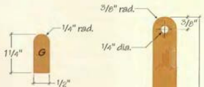
END VIEW FEED DAMS
