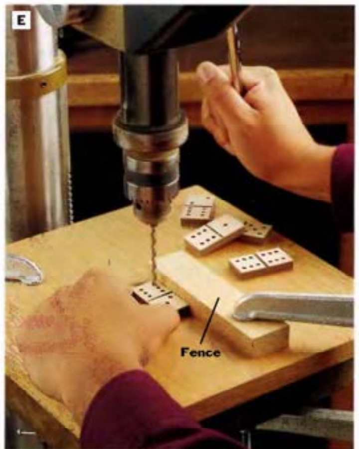
PHOTO E: Drill shallow holes through the maple veneer and just into the walnut core to create the domino dots. Set the depth stop to keep the bit from drilling too deeply. Clamp a fence to the drill press table so the rows of dots will line up lengthwise along the dominoes. Work carefully when drilling to hit your dot locations precisely.
