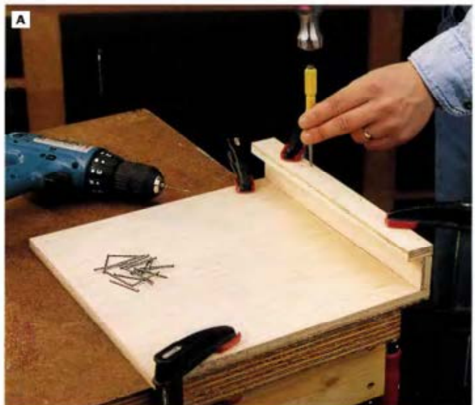
PHOTO A: Assemble the book rest, shelf and shelf lip with glue and 1 1 / 4 -in. finish nails. Drill pilot holes first for the nails.
