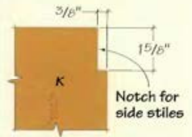
CHEST BOTTOMS
