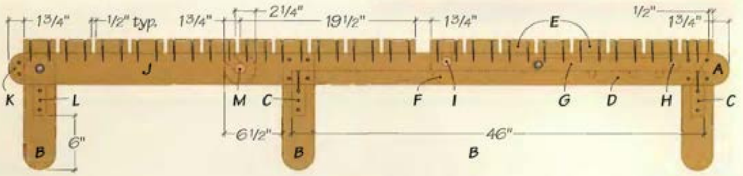
SIDE VIEW
