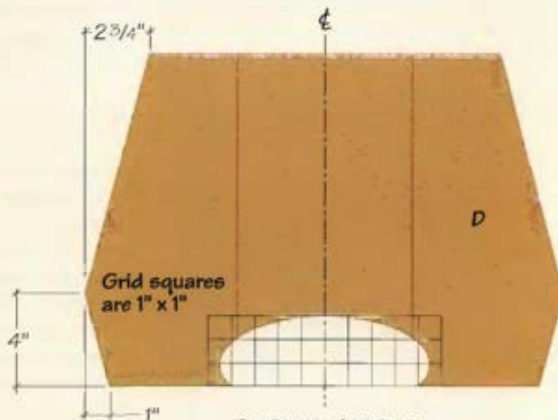
DECK PLANTER
