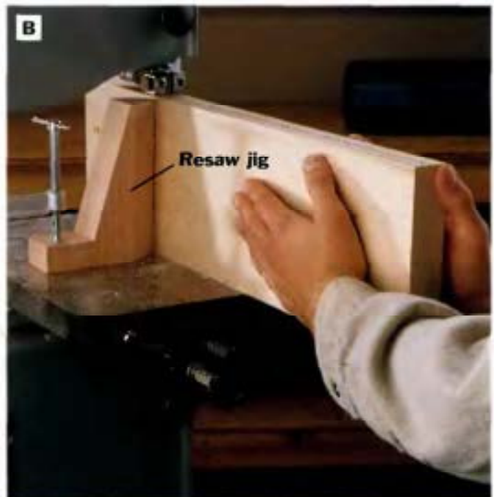
PHOTO B: Resaw the maple stock in half for the sides and ends of the box, using a marked centerline as a guide for the blade. A shop-made resaw jig clamped to the saw table will help square the board to the table and keep the blade tracking along the cutting line.
