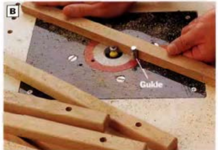
PHOTO B: Ease the edges and ends of the slats and crossbars with a 1/8-in. roundover bit in the router table. Use a pin-style guide on the router table to help control the workpieces as you machine them.
