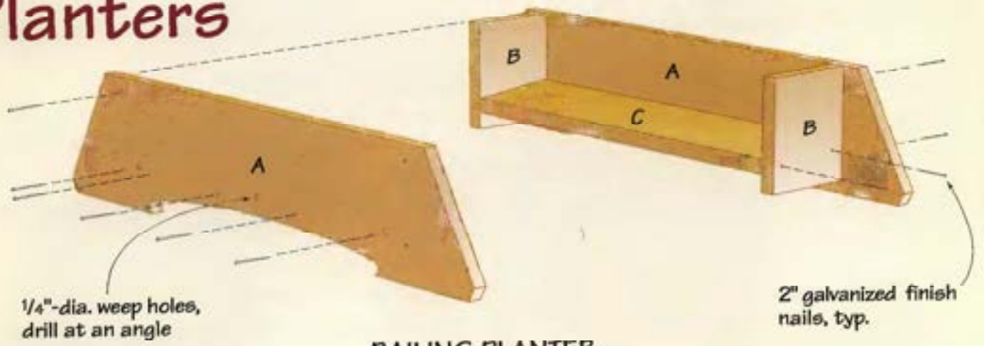
RAILING PLANTER
