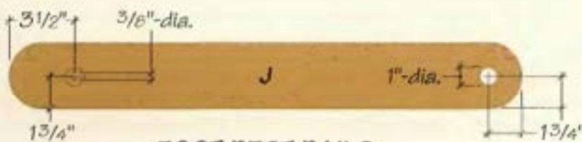
FOOT REST RAILS
