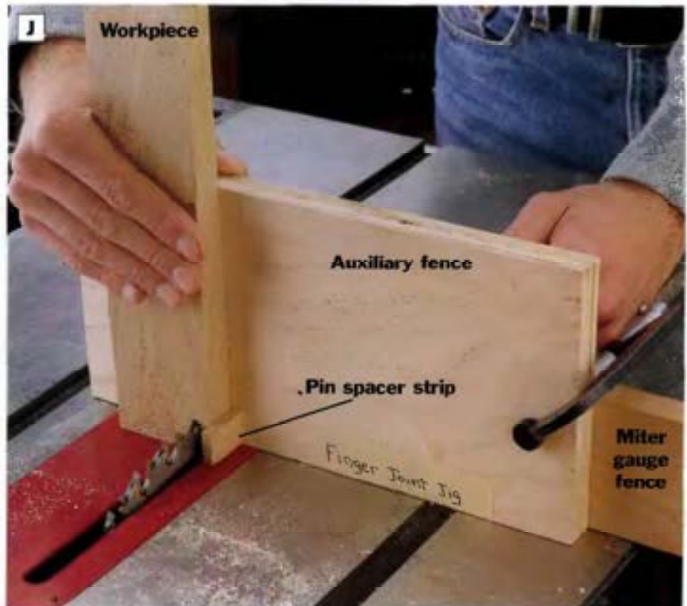
PHOTO J: The jig we used consists of an auxiliary fence clamped to the miter gauge fence. A \frac{3}{4} -in.-wide \times \frac{3}{16} -in.-deep slot in the auxiliary fence is filled with a pin spacer strip to use as a gauge for aligning the finger joint cuts. Make the first finger joint cut with the workpiece butted against the pin spacer strip.
