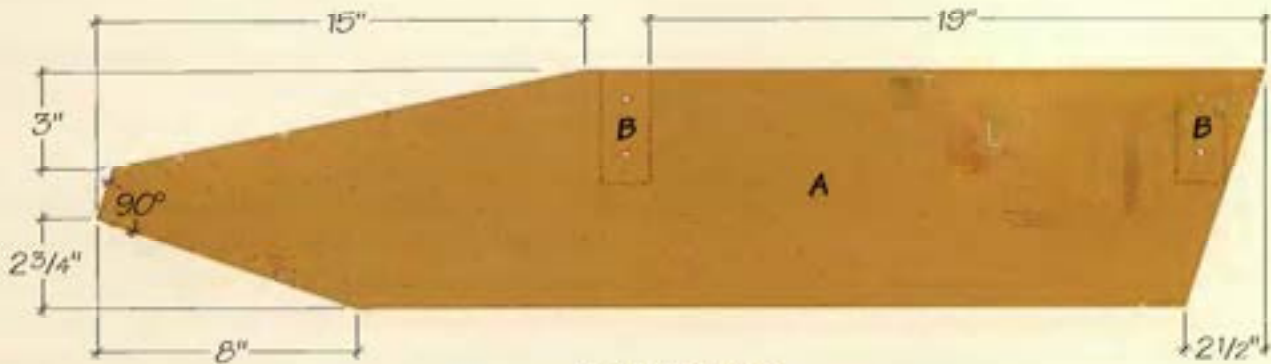
BACK LEGS
